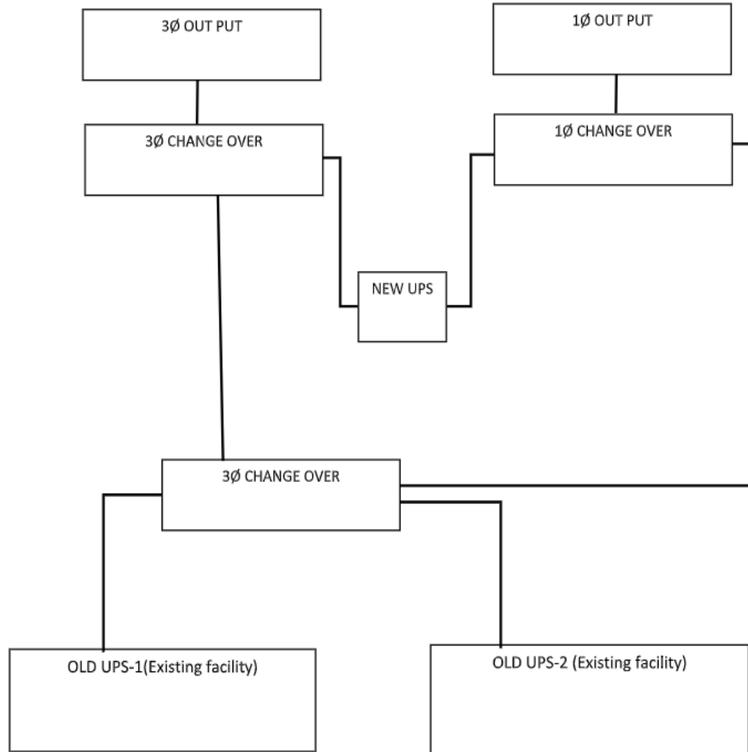
Single Line Circuit Diagram
