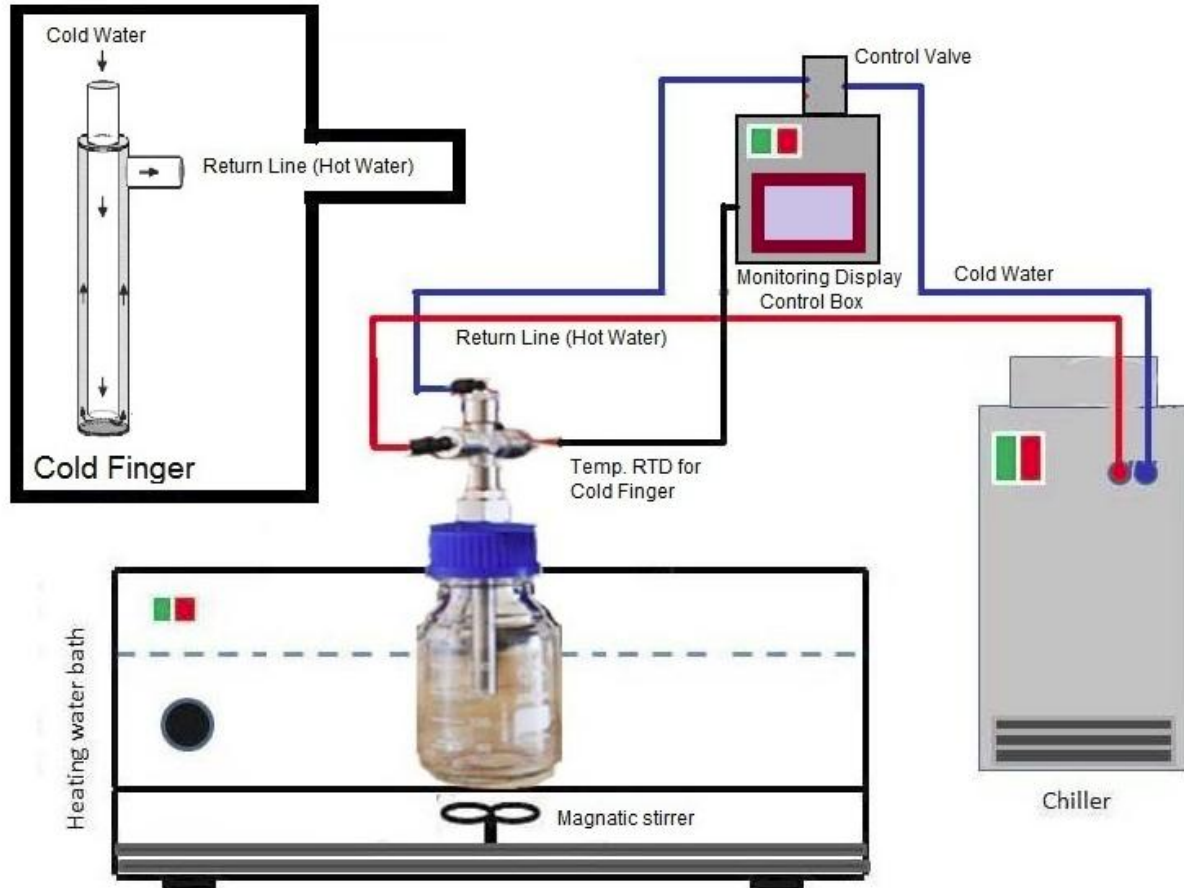
Schematic of Wax Deposition Set up
